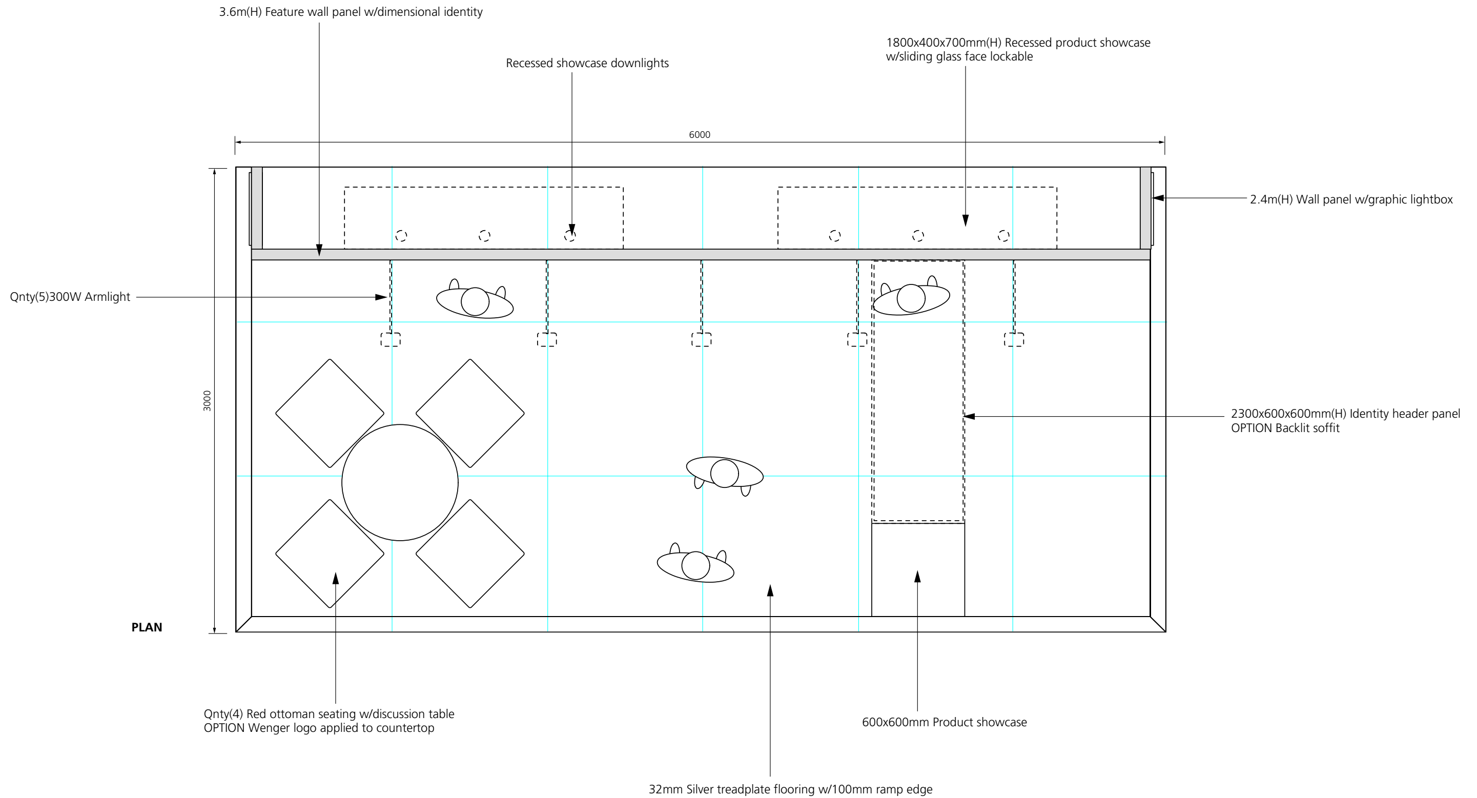
6Mx3M Floorplan Scale 1:25/A3
